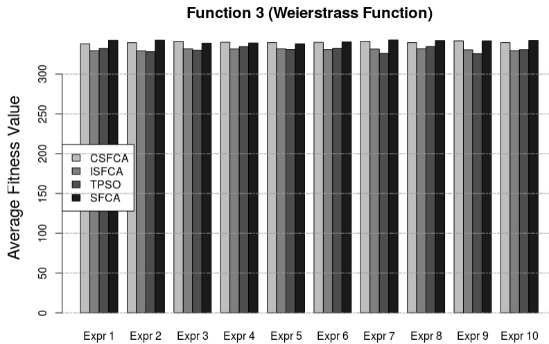
Figure 6.6: Average fitness values for Function 3 with 30 dimensions
